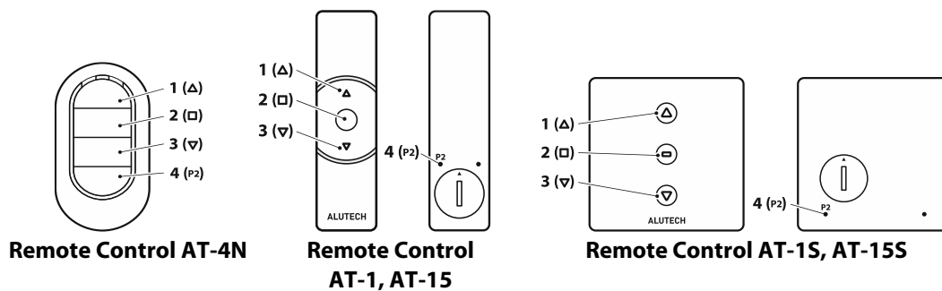
Fig.2 – The appearance of remote controls and key purpose: 1 – Up Key; 2 – Stop Key; 3 –Down Key; 4 – Programming Key.
